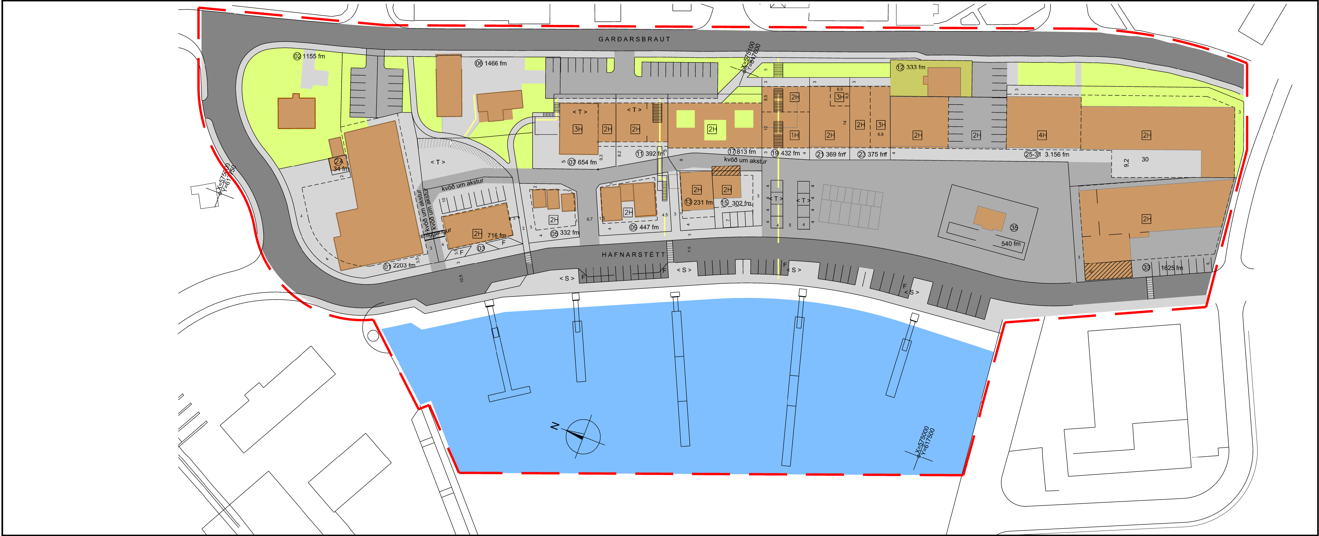
GILDANDI DEILISKIPULAG Mkv. 1:750 (A1)
